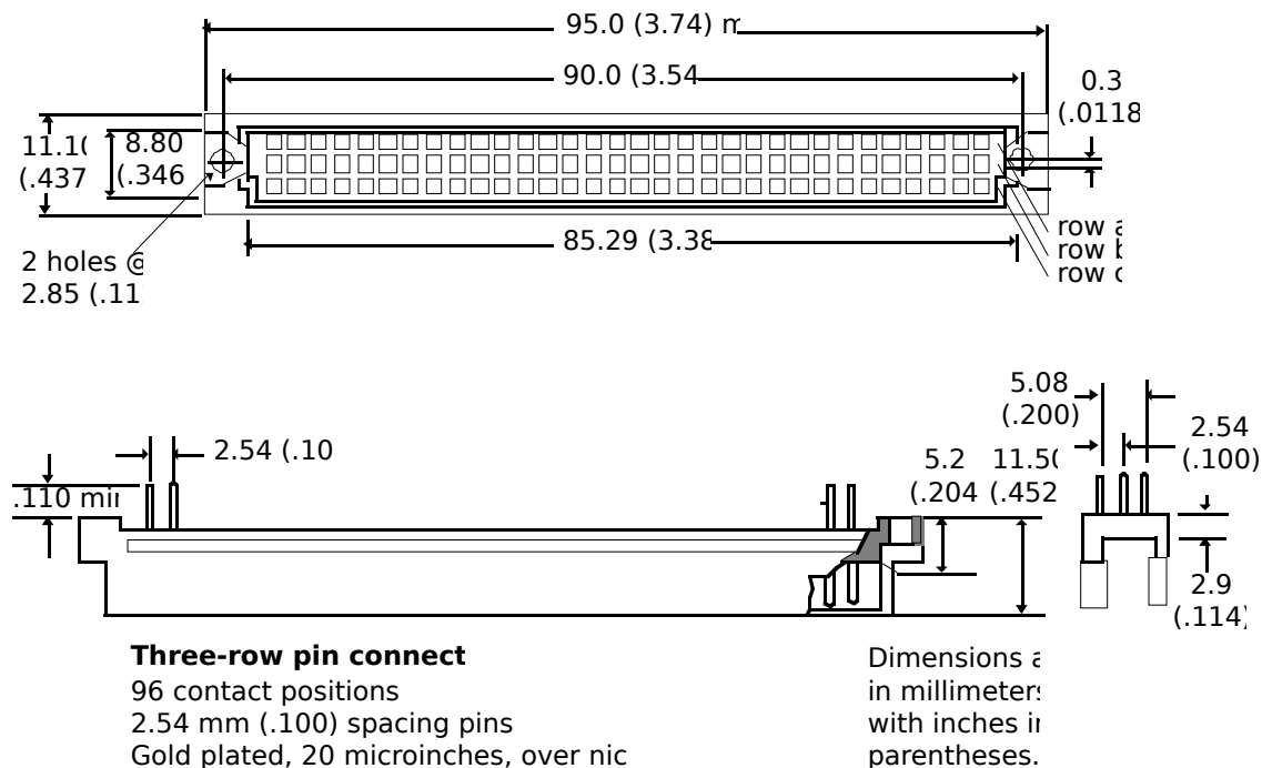
Figure 1—96-Pin Plug Connector
